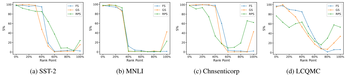
Figure 2: Completeness performance of evaluated IA methods. We report the S% of each rank point on the four evaluated datasets. All the reported results are averaged over 5 different runs.
