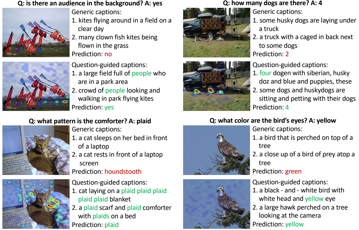
Figure 2: Examples of generic captions (from all patches) based on the original image and question-guided captions (from the sampled patches) based on the GradCAM heatmaps on VQA v2 data. For illustrative purposes, we highlight words in green to indicate correct answer predictions and the cues from captions. Words in red indicate wrong answer predictions.
