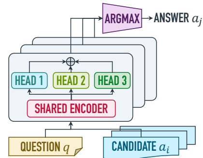
Figure 1: CERBERUS model for answer sentence selection. The model consists of a shared encoder body and multiple ranking heads. CERBERUS independently scores up to hundreds candidate answers a_i for question q ; The one with highest likelihood is selected as answer.
