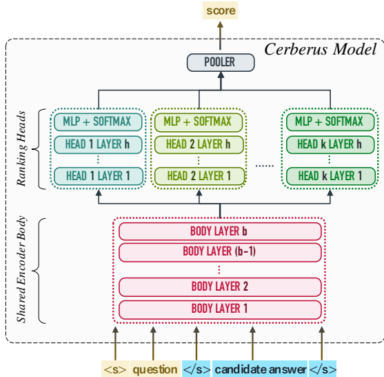
Figure 2: Detailed overview of CERBERUS model that consists of a shared encoder body of b transformer layers, followed by k ranking heads of h layers each; we use notation B_b kH_h to identify a CERBERUS configuration. All heads are jointly trained, but each head learns from a unique teacher model ; at inference time, predictions from heads are combined by a pooler layer.
