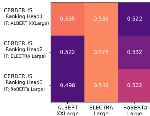
Figure 3: Agreement between heads and their teacher model in CERBERUS. It is obtained by dividing the number of correct candidates each head and teacher agree on by the total number of correct answer for each head.
