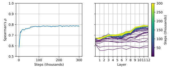
Figure 2: Analysis of STS learning dynamics. Left : Spearman correlation after fine-tuning with various checkpoints. Right : Spearman correlation on all the layers with selected checkpoints. Each line represents one checkpoint and its results on all the layers.
