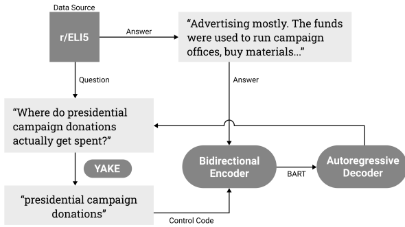
Figure 2: Architecture to train the CONSISTENT model
