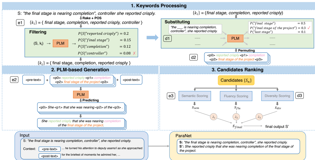
Figure 2: The complete generation process of Paraphrase Machine. The keywords filtering, substitution, PLM-based generation, and candidate evaluation steps are all achieved with PLMs in an unsupervised manner.
