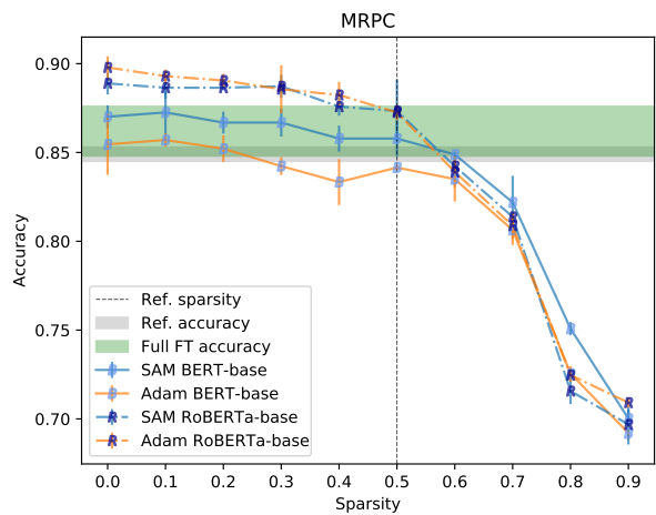
(b) MRPC, IMP w/ RoBERTa base
