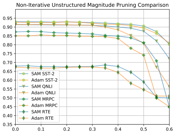
Figure 7: SAM- and Adam-optimized models evaluated directly after pruning a proportion of parameters from the full-sized model. Models fine-tuned with SAM hold up better to non-iterative magnitude pruning as well.
