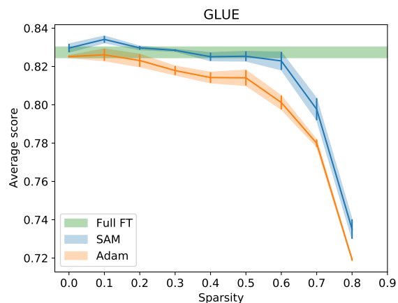
Figure 1: Average score over all GLUE tasks as a function of sparsity (% of parameters pruned) of BERT base through unstructured iterative magnitude pruning. We compare the baseline Adam optimized model’s performance to our model, optimized to prefer flat minima via SAM. The green horizontal bands mark initial performance of our full fine-tuned (FT) models. SAM outperforms baseline Adam across all sparsity values.
