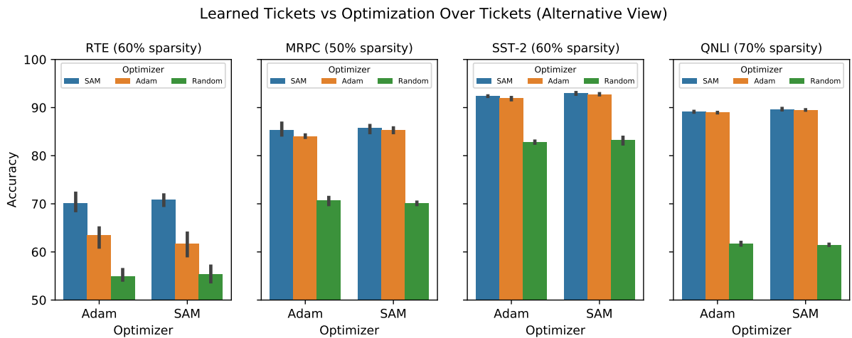
Figure 12: An alternative view of the same information contained in Figure 3. Note that, for example, in RTE, SAM tickets clearly outperform vanilla Adam tickets regardless of the optimizer used for the final fine-tuning.
