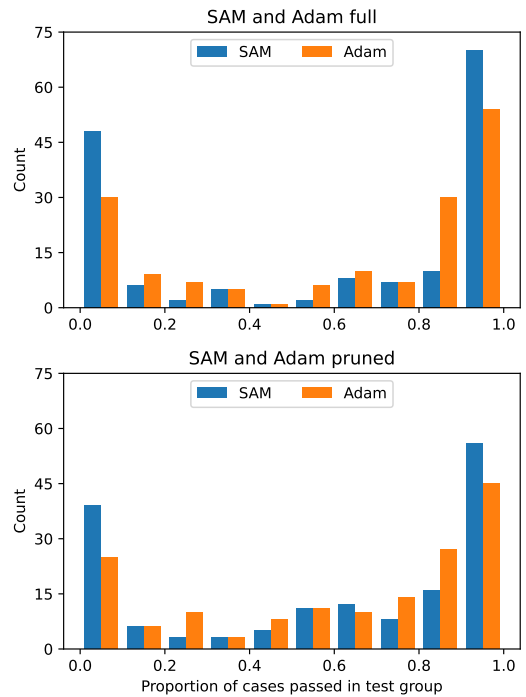
Figure 16: Aggregated Checklist (Ribeiro et al., 2020) results for QQP models. Tests target various capabilities of models such as robustness to typos and simple coreference resolution. Note the concentration of frequencies near 0.0 and 1.0 for all models, as well as the shifts in frequencies when pruned for both vanilla Adam and SAM models; models can effectively lose or even gain specific capabilities throughout compression.
