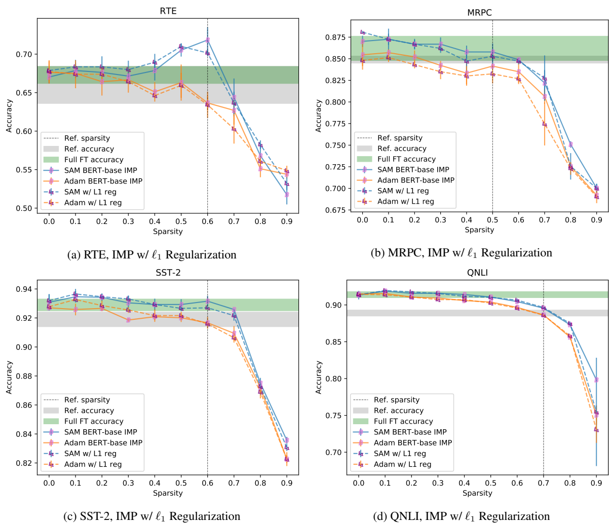
Figure 10: Individual plots showing sparsity vs. accuracy for GLUE tasks in \ell_1 -regularized BERT base models compressed with iterative magnitude pruning (IMP), with regular BERT base models for comparison. The vertical lines and gray horizontal bands mark reference sparsity and "winning ticket" evaluation metric values that were obtained by Chen et al. (2020) . The green horizontal bands mark the initial performance of our full fine-tuned models.
