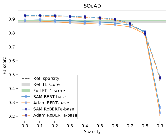
(e) SQuAD, IMP w/ RoBERTa base
