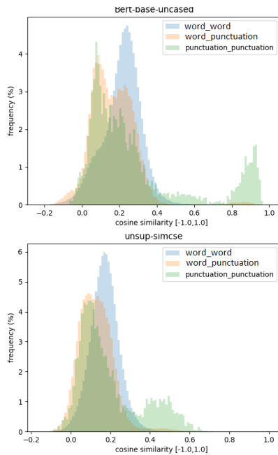
Figure 3: Cosine similarity between punctuation marks and other tokens from uncased BERT (top) and unsupervised SIMCSE (bottom)
