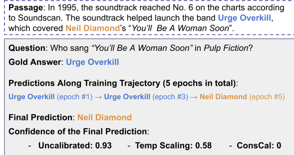
Figure 4: An example from NQ where the final prediction is wrong. The original uncalibrated confidence is over-confident, while temperature scaling lowers the confidence, it is still over-confident and could mislead users. CONSCAL sets the confidence to 0 because predictions across checkpoints in the training trajectory are inconsistent—the model is confused between the specific performer and the original singer in this example.
