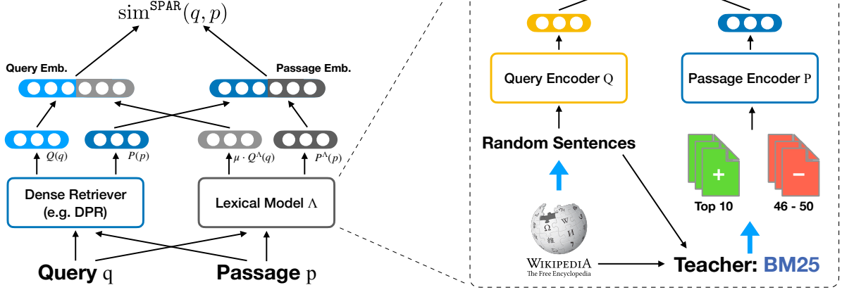
Figure 1: SPAR augments a dense retriever with a dense Lexical Model \Lambda trained to imitate a sparse teacher retriever. \Lambda is trained using random sentences as queries with positive and negative passages produced by the teacher. \Lambda is then combined with a dense retriever via vector concatenation to form a salient-phrase aware retriever.
