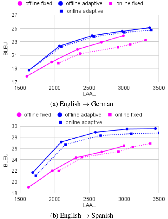
Figure 4: LAAL-BLEU curves of offline- and simultaneous-trained Conformer models with sequence-level KD.
