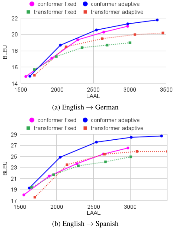
Figure 3: LAAL-BLEU curves of the Transformer- and Conformer-based architectures.
