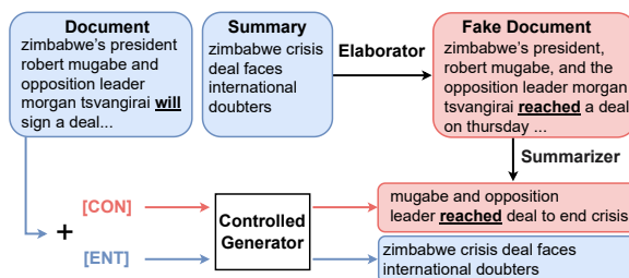
Figure 1: Overview of CoFE. The original and fabricated document-summary pairs are shown in blue and red respectively. The trained elaborator first generates fake documents from the summary. Then, the summarizer generates summaries from the fake documents, which are likely to contain hallucinated information (underlined). A controlled generator is then trained to produce the original (faithful) and the fabricated (unfaithful) summaries depending on the control codes.
