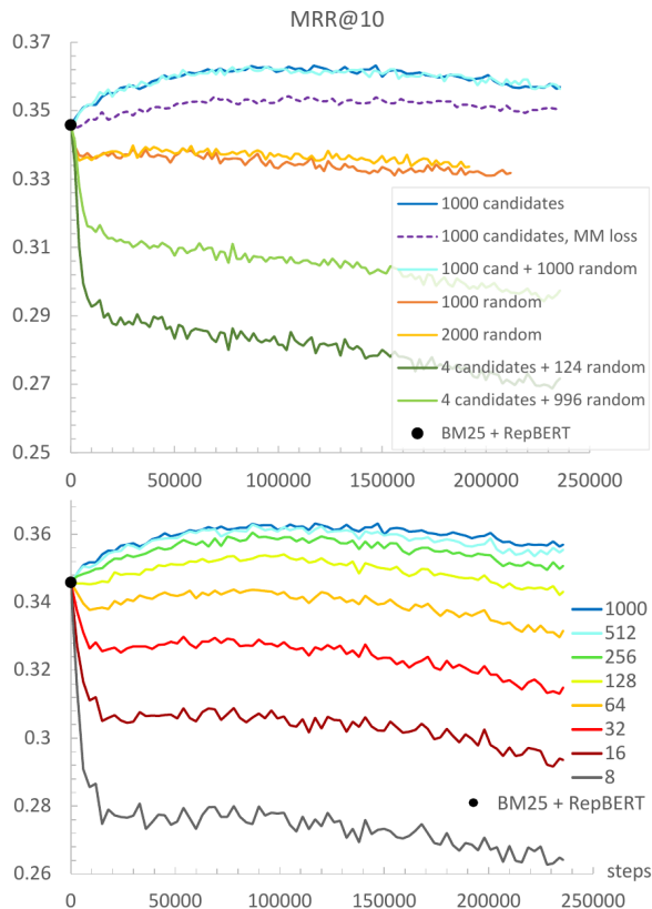
Figure 2: Performance of BM25→CODER(RepBERT) on MS MARCO validation set over training steps. The left-most point corresponds to reranking BM25 candidates using the fully trained RepBERT. Top: Effect of type and number of documents used as negatives. The purple dashed curve corresponds to training with a pair-wise (Max Margin) loss. Bottom: Effect of number of BM25 candidates used as negatives during training.
