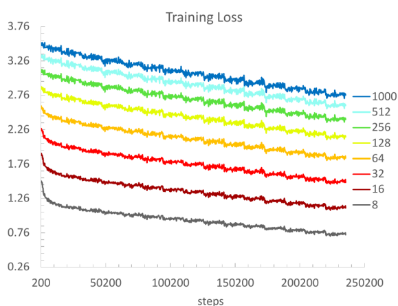
Figure 6: Evolution of the loss on the training set, as training of BM25→CODER(RepBERT) progresses. Different curves correspond to a different number of BM25 candidates used as negatives during training. While training loss is decreasing in all cases, only using a large number of candidates results in a significant improvement of performance over the base method on the validation and test sets (see Figure 2).
