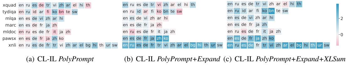
Figure 7: The relative performance improvement at the language level for PolyPrompt with cross-lingual prompts (CL) versus in-lingual prompts (IL). Languages are sorted in descending order according to the sample size of the languages in the mT5 training set (high-resource to low-resource from left to right). The bluer (redder) the color, the greater the improvement (decrease) of CL over IL.
