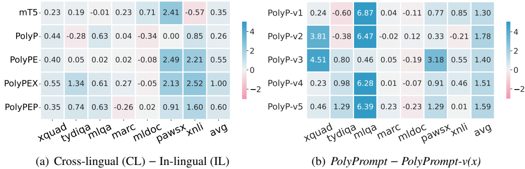
Figure 5: The exploration of the language and uniformity of prompt design. (a) is the performance gap between cross-lingual (CL) and in-lingual (IL) prompt templates, where PolyP , PolyPE , PolyPEX , and PolyPEP are abbreviations for PolyPrompt , PolyPrompt+Expand , PolyPrompt+Expand+XLSum , and PolyPrompt+Expand+PANX . (b) is the relative performance improvement of PolyPrompt with unified prompt templates versus diversified prompt templates (e.g. PolyP-v1 ). PolyP-v(x) ( x \in [1, 5] ) represent x -th version of diversified prompt templates. The bluer color indicates that the model with the cross-lingual (unified) prompts outperforms the in-lingual (diversified) prompts more, while the redder color has the opposite meaning. The last column is the average relative improvement.
