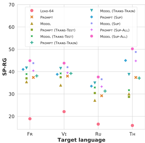
Figure 4: SP-ROUGE scores of our baselines (LEAD-64, PROMPT-TUNING, MODEL-TUNING) at the XXL model size, in the zero-shot XGEN setting. For comparison, we also show the headroom available if a machine translation system is used (TRANS-TRAIN, TRANS-TEST), or if gold data in target languages is used (SUP, SUP-ALL).
