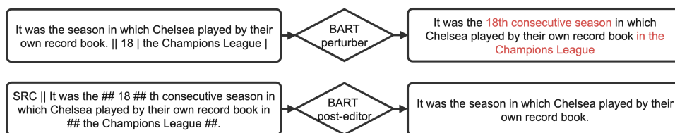
Figure 1: Overview of our compression-based approach. A perturber model is trained to produce an uncompressed sentence with inserted entities, conditioned upon the compressed sentence and an appended list of entities. The perturber is applied to a dataset’s reference summaries to create data to train a post-editor that takes the document (SRC) and a summary with entities to remove surrounded by special tokens, and removes the erroneous words.
