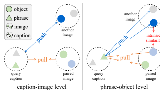
Figure 1: Previous methods neglect the intrinsic similarity which can be seen as a soft co-occurrence. Utilizing the intrinsic similarity between negative examples (dark blue circle) and false-positive examples (light blue circle) can push the false-positive examples away from the query phrase (light green triangle).
