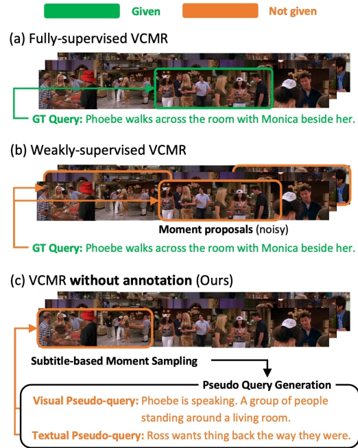
Figure 1: Comparison with different supervision settings in VCMR. (a) Fully-supervised VCMR (paired video query with timestamp), (b) Weakly-supervised VCMR (paired video query without timestamp), (c) VCMR without annotation (unlabeled video).
