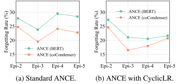
Figure 4: Fraction of training queries the models performed worse after one training episode, compared with their MRR@100 in the past episode.
