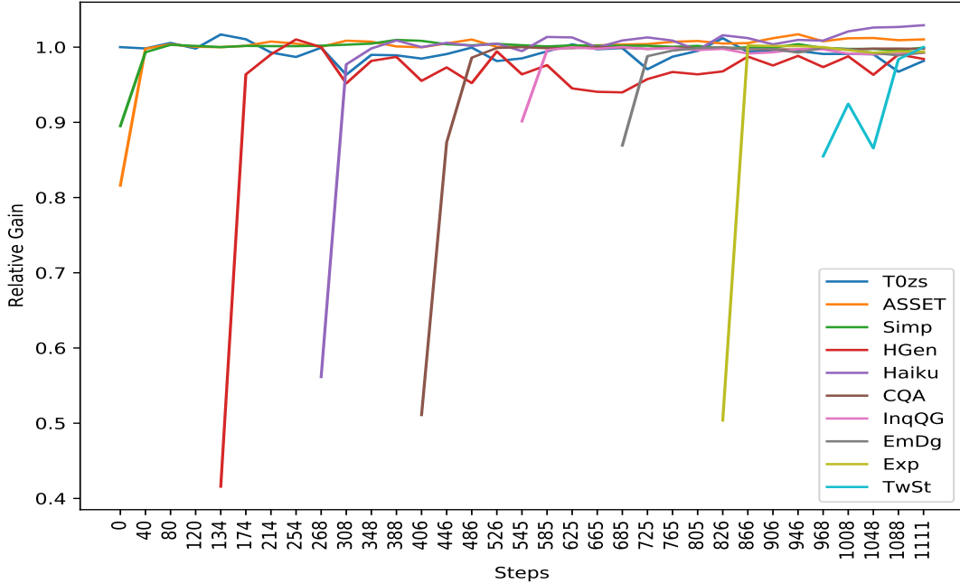
Figure 2: Progressive Relative Gain results for CT0 (11B) during the sequential learning (Y axis) vs Number of Training steps (X axis). The curves for tasks T_0, \dots, T_7 are displayed respectively at step 0, ..., i such that only the first task, Simplification (green and orange) is present at step 0, then HGen (red) etc.
