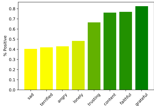
Figure 3: Emotion Generalization: Percentage of Haiku classified as positive, when adding emotion specific constraints to the Haiku instruction. We used an open source binary sentiment analysis classifier. 6
