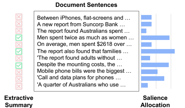
Figure 1: Illustration of different guidance. Extractive summary is a strict guidance consisting of extracted sentences labeled with check-mark. Salience allocation is a flexible guidance mapping sentences to different salience degrees shown as a bar chart.
