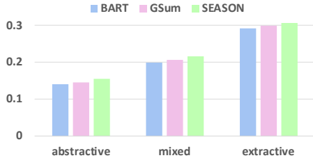
Figure 3: R-2 scores by density on CNNDM test set.
