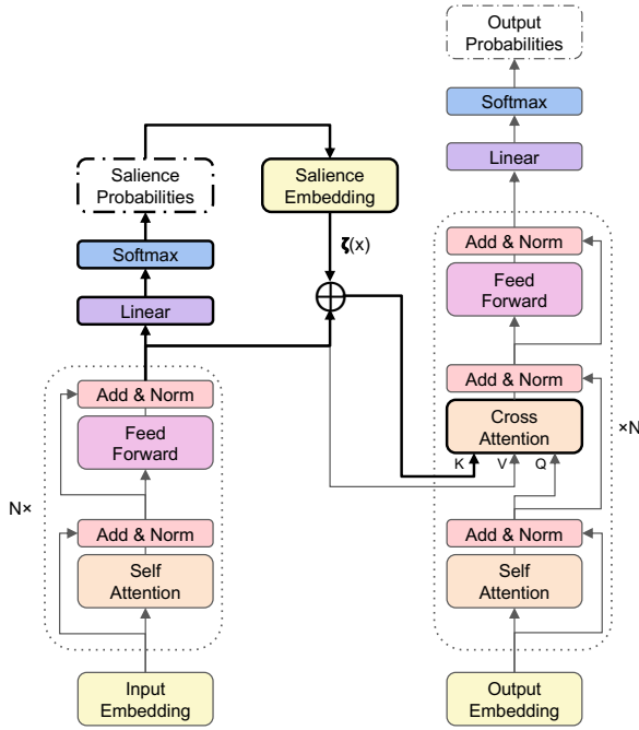
Figure 2: Model architecture of SEASON. The proposed modules are highlighted with bold lines. SEASON adds a saliency predictor on top of the encoder, maps (the expectation of) saliency degrees to corresponding embeddings, and adds these saliency embeddings to the key vectors of cross attention.
