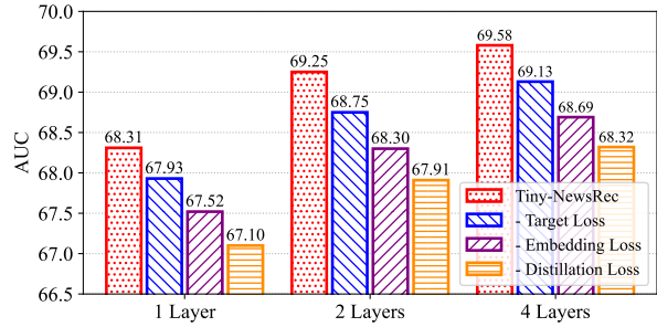
Figure 4: Effectiveness of each loss function.
