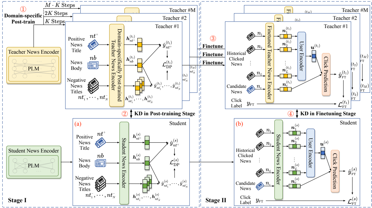
Figure 1: The framework of Tiny-NewsRec
