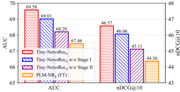
Figure 3: Effectiveness of each stage in our framework.
