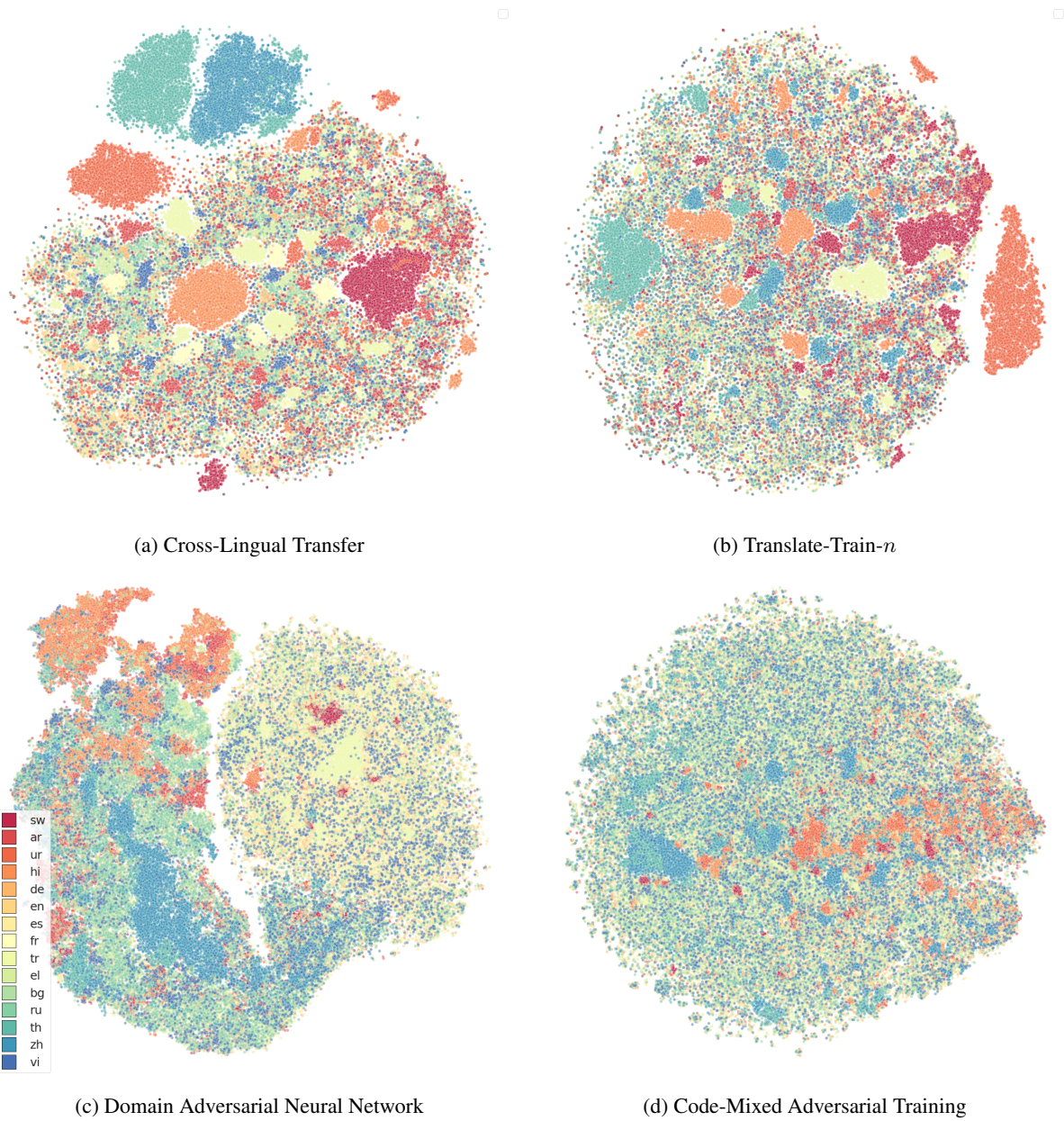
Figure 5: t-SNE visualizations of XLM-R base representations fine-tuned using different methods. Here, we average all the token embeddings in the sentence instead of just using the <math>\langle s \rangle</math> embedding.
