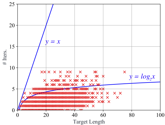
Figure 4: # Iters. vs. length of target sentences with respect to the different instances (denoted as \times ) on WMT14 En \rightarrow De test set.
