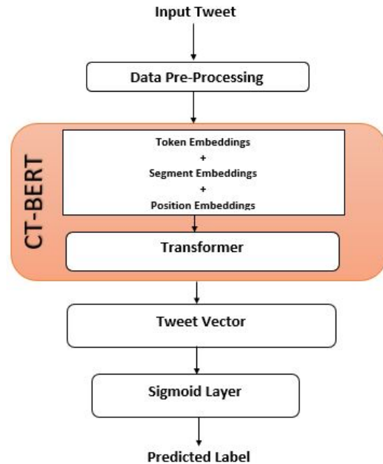
Figure 1: Overview of Model-1
