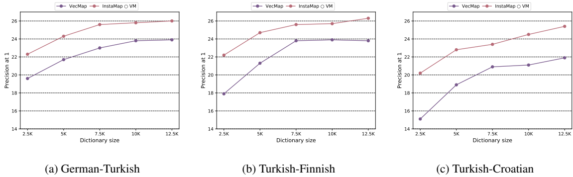
Figure 2: Comparison of performance between VECMAP and INSTAMAP applied on top it (IM ◊ VM) for different sizes of the training dictionary (from 2.5K word pairs to 12.5K word pairs in steps of 2.5K pairs).
