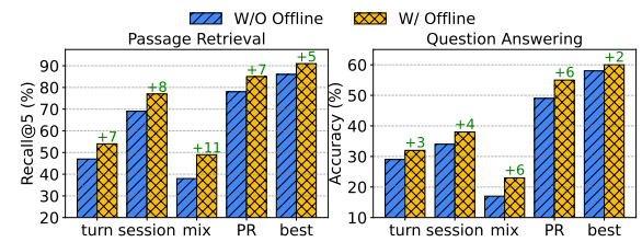
Figure 5: Impact of offline pretraining on retriever performance for LongMemEval dataset with the same 100 random samples as Figure 4. Results without offline pretraining are shown in blue, while results with offline pretraining are shown in orange. Offline pretraining improves recall and accuracy across all settings.
