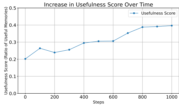
Figure 6: Convergence of usefulness scores (ratio of useful memories cited) over RL training steps. The score improves as the reranker is updated based on Retrospective Reflection, indicating enhanced alignment between retrieved memory and generated responses.
