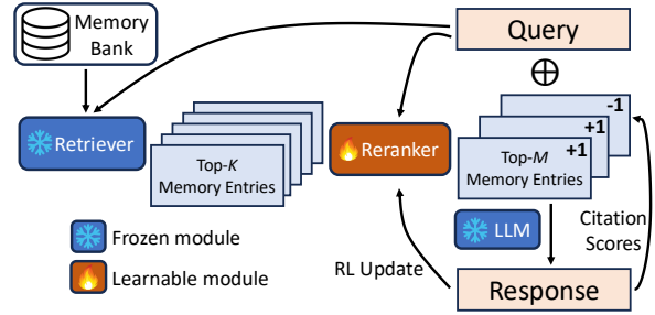
Figure 3: Illustration of Retrospective Reflection . The Retriever fetches Top- K memory entries from the memory bank, which are refined by the learnable Reranker to select the Top- M most relevant entries. These entries are passed to the LLM along with the query to generate the final response. The LLM assigns binary citation scores ( +1 for useful and -1 for not useful) to the retrieved memory entries based on their utility in the response. These scores are used as reward signals to update the reranker via an RL update , adapting the selection of relevant memory over time.
