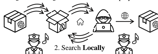
Figure 1: Unlike mainstream black-box attack methods that repeatedly probe the target model with malicious instructions, ShadowBreak reduces detection risk by conducting searches on a local mirror model. This mirror model is aligned using benign distillation data from the target model, a process designed to bypass content moderation. The resulting prompts are then transferred to the target model.
