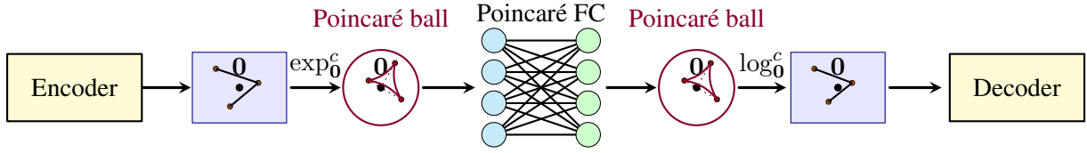
Figure 2: Model architecture for our approach. After the T5 encoder, we project the resulting Euclidean embeddings onto the Poincaré ball. These hyperbolic embeddings are then refined through a trainable Poincaré layer. For compatibility with the T5 decoder, we project the hyperbolic embeddings back to the Euclidean space. While the T5 encoder and decoder parameters remain frozen throughout the training, the input contains trainable soft prompts.
