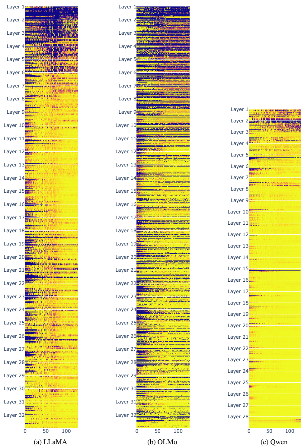
Figure 6: Visualizing the utilizatio score for the dimensions in the query vectors.
