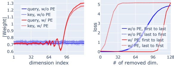
(a) The average magnitude of the key and the query vectors for each dimension. (b) # of removed dimensions v.s. loss in Eq. 2 ( -\mathbb{E} \log P(v_i|q_i, K, V) ).
