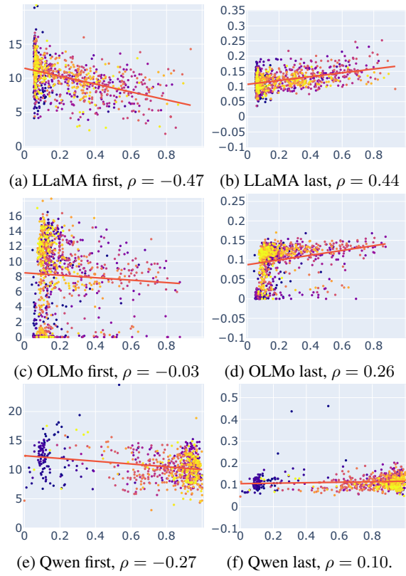
Figure 4: The relationship between the L1 norm of rows in query projection matrices (x-axis) and the utility scores of the first or last dimensions (y-axis). Each dot represents an attention head. The lighter dot color represents the deeper layers. The red line represents the linear regressor.
