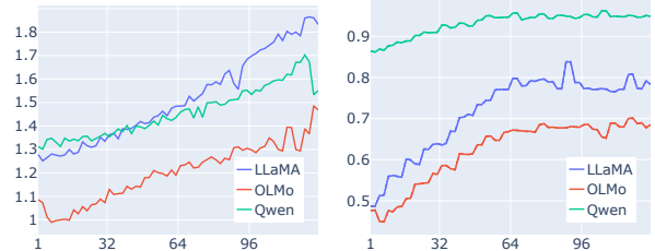
(a) Average L1 norm (b) Average utility score.
