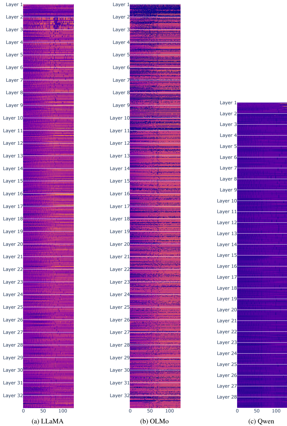
Figure 5: Visualizing the L1 norm of the rows in the query projection matrices.
