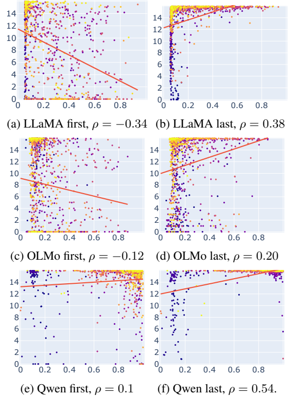
Figure 3: The relationship between the retrieval-head indicator score (x-axis) and utility score of the first 16 or last dimensions (y-axis). Each dot represents an attention head. The lighter dot color represents the deeper layers. The red line represents the linear regressor.
