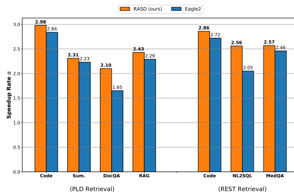
Figure 1: Speedup Performance of EAGLE2 vs. RASD with PLD and REST Retrieval Methods on Qwen2.5-14B.
