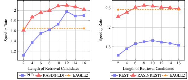
Figure 3: RASD performance with different lengths of retrieval candidates compared with the baselines
