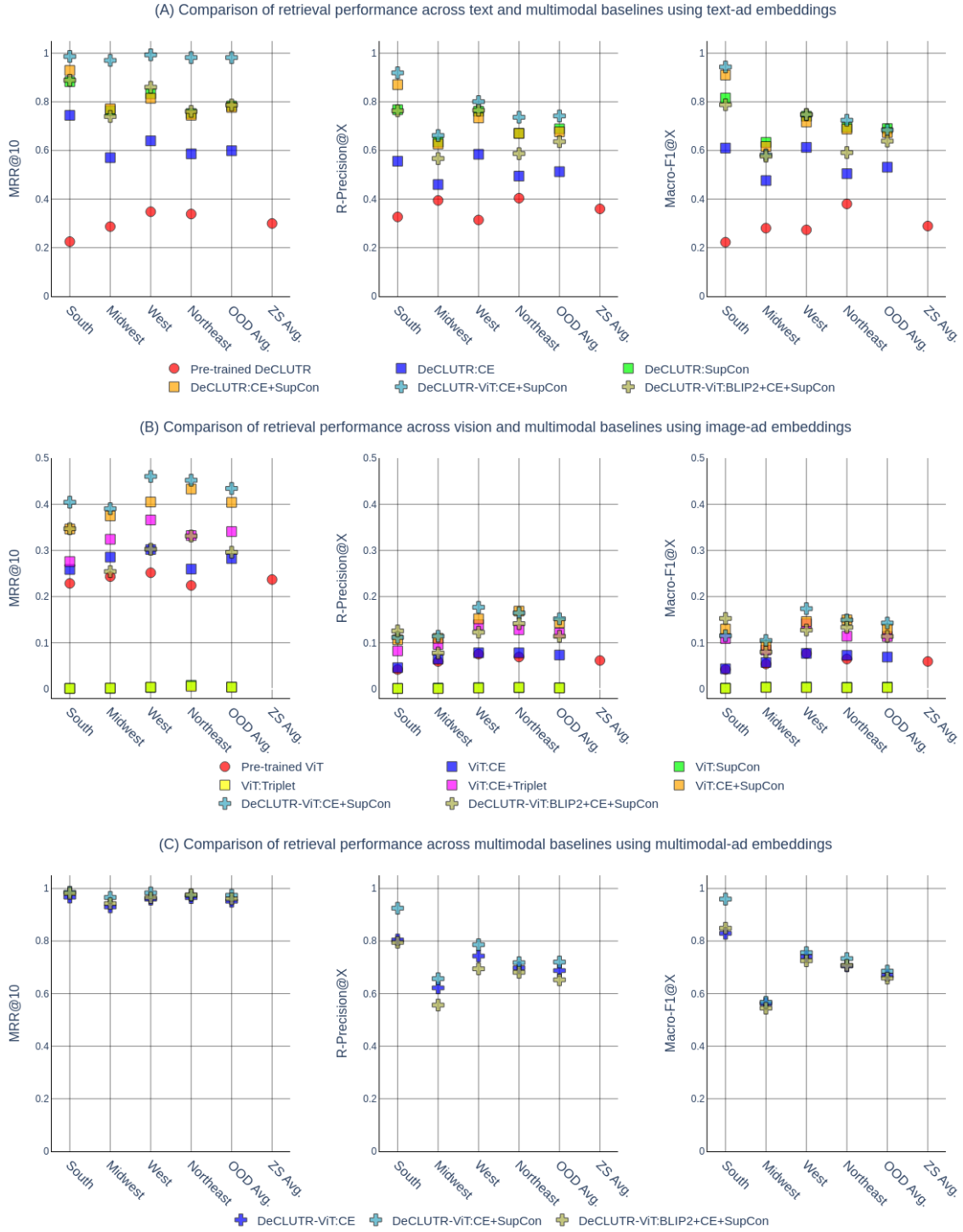
Figure 1: Comparison of retrieval performance across multiple baselines for text-to-text, image-to-image, and multimodal ads retrieval tasks on South, Midwest, West, and Northeast datasets. The text-to-text retrieval baselines include the pre-trained DeCLUTR checkpoint (●), DeCLUTR classifiers trained on CE (■) and CE+SupCon losses (■), and the DeCLUTR backbone trained with SupCon loss (■). Image-to-image retrieval baselines include the pre-trained ViT checkpoint (●), ViT classifiers trained on CE (■), CE+Triplet (■), and CE+SupCon losses (■), and ViT backbones trained with SupCon (■) and Triplet (■) losses. Multimodal baselines include End2End DeCLUTR-ViT classifiers trained with CE (⊕), CE+SupCon (⊕), and BLIP2-aligned DeCLUTR-ViT classifiers trained with CE+SupCon (⊕) objectives.
