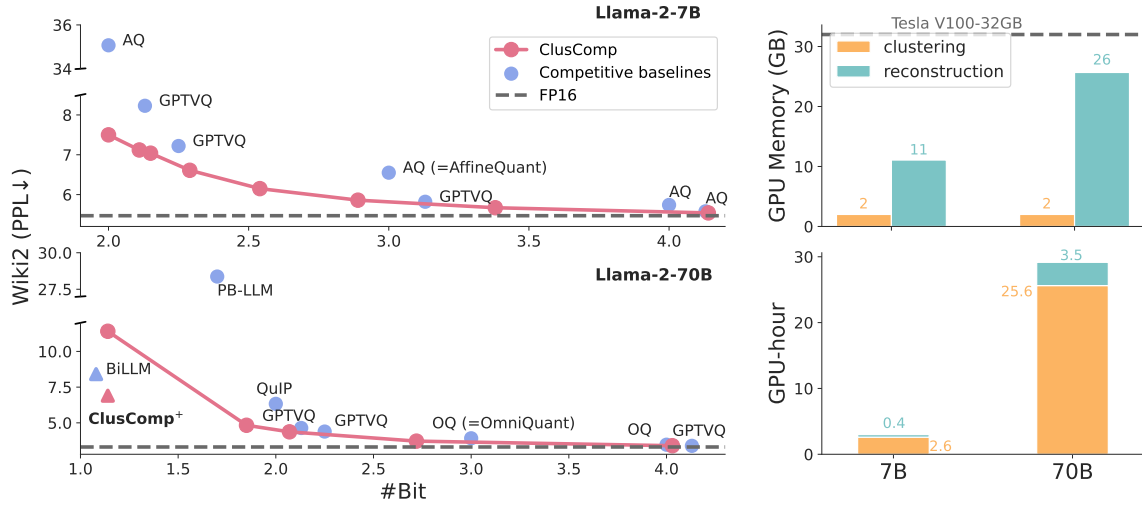
Figure 1: Left: Compression quality of ClusComp. Only the most competitive baselines are shown here. Please refer to Table A.1 and A.2 for a full comparison. Methods in triangle use more calibration samples than the ones in circle. Right: Compression efficiency of ClusComp that consists of sequential clustering and reconstruction steps. E.g., compressing a 70B LLM takes 25.6h + 2GB for clustering, and 3.5h + 26GB for reconstruction on 1 GPU.
