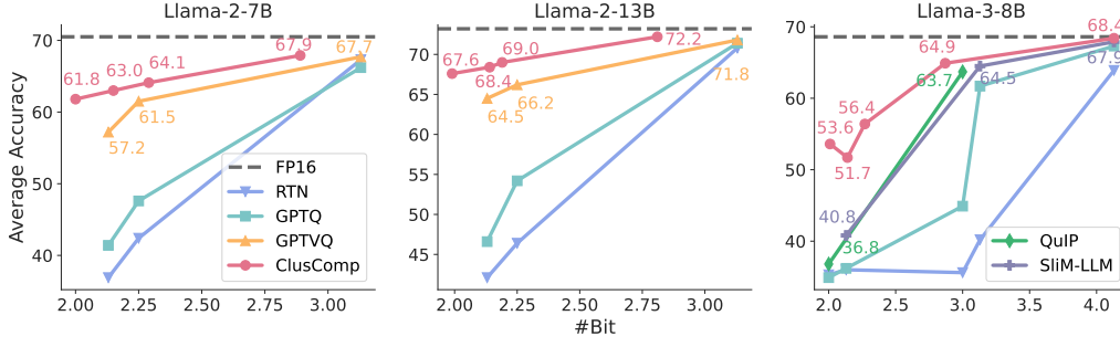
Figure 3: Average zero-shot accuracy over 5 or 6 commonsense reasoning tasks, only including competitive baselines. Please refer to Table A.3 and A.4 for detailed numbers and the full comparison.
