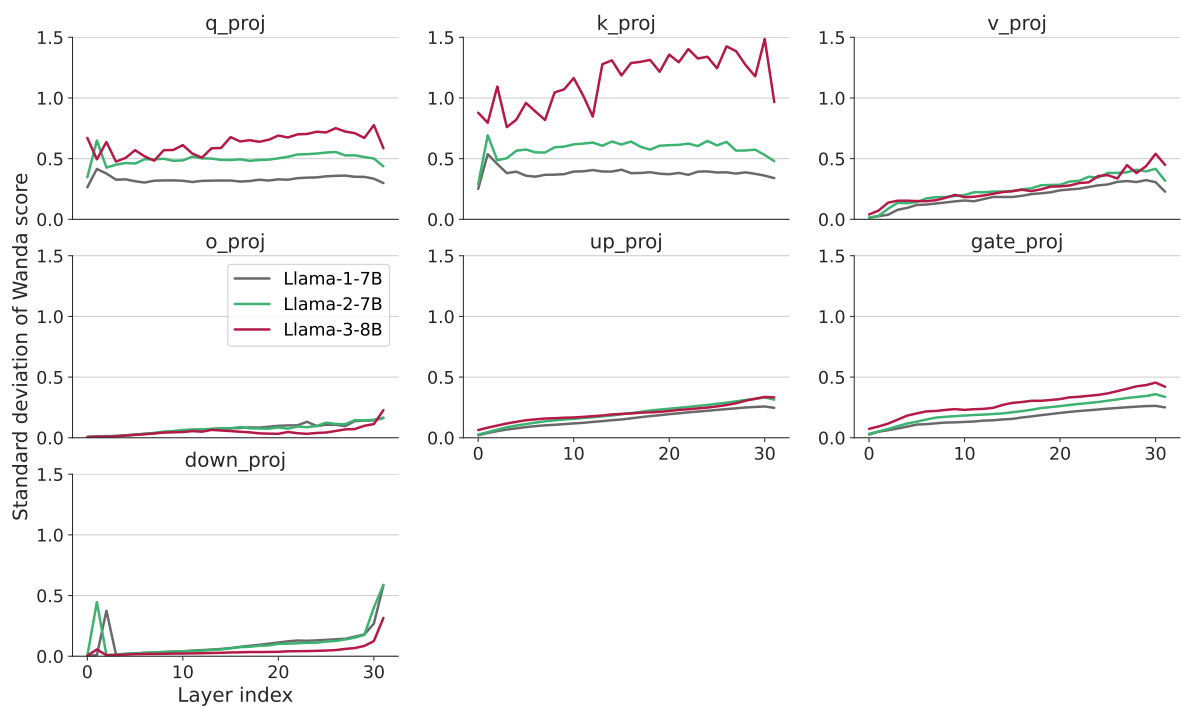
Figure B.2: The standard deviation of Wanda score across various layers in different Llama series reveals three key observations: (1) Deeper layers tend to exhibit higher standard deviation; (2) Three layers (query, key and gate) show a clear trend across Llama series, with Llama-3 showing the highest standard deviation, followed by Llama-2, and then Llama-1; (3) The other four layers show a similar standard deviation for all Llama series.
