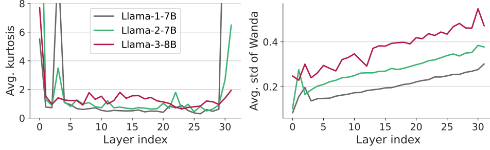
Figure A.1: From Llama-1 to Llama-3, LLMs exhibit increasing challenges for quantization. Left: The average kurtosis of weights across various layers in the Llama series, previously shown in Figure 2 (Right). Please refer to Figure B.1 for the kurtosis of different layer types. Right: The average standard deviation of the Wanda score across various layers. Please refer to Figure B.2 for the Wanda scores of different layer types. Both metrics indicate that Llama-3 has higher variance in most layers, reflecting the presence of more outliers and thus greater difficulty for quantization.
