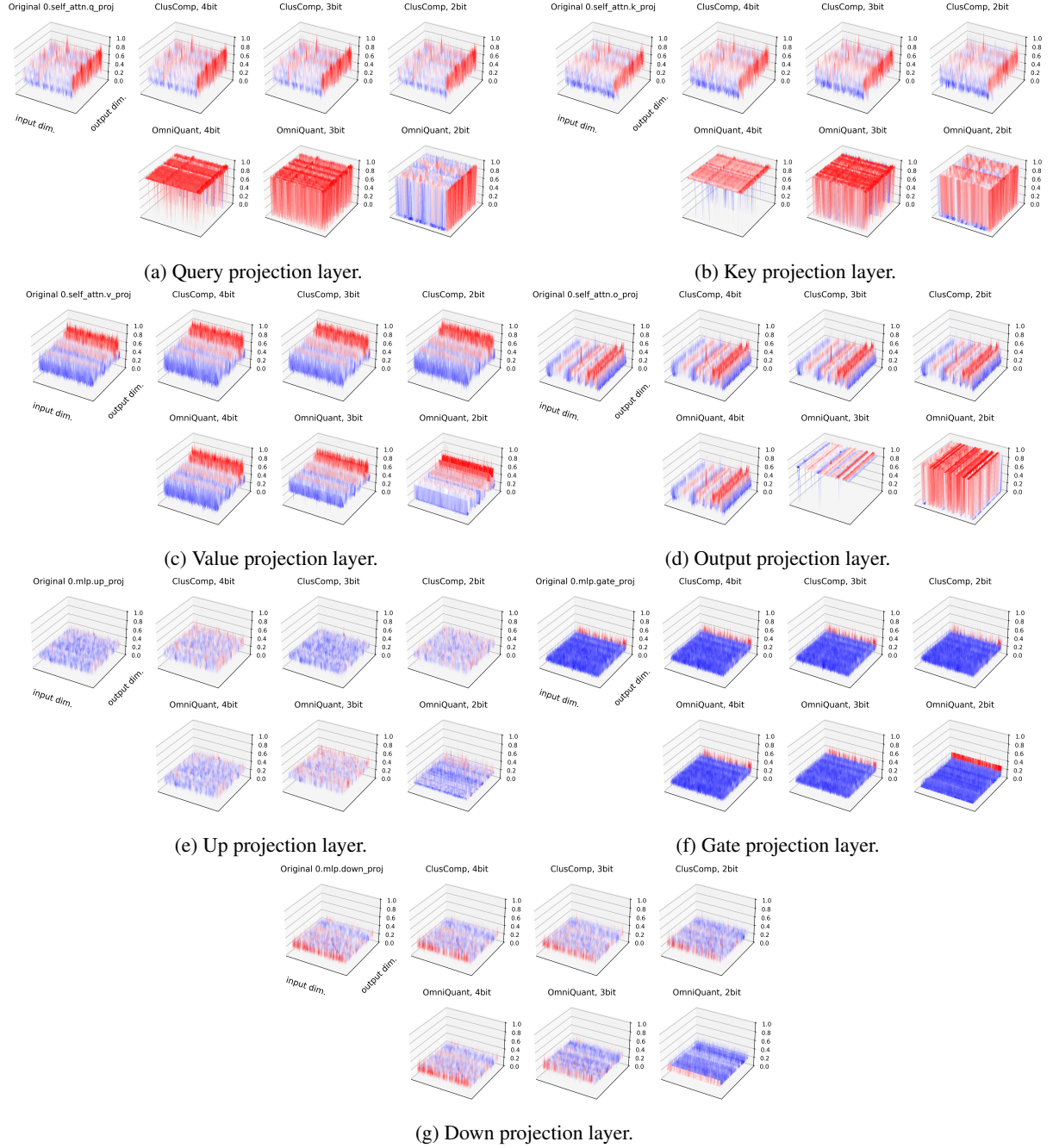
Figure A.3: Weight patterns of all layers in the first block (0-th block) of Llama-2-7B. Darker red and blue indicate larger and smaller weight values, respectively. ClusComp’s weight distribution of different bit levels can better simulate the original weight distribution.
