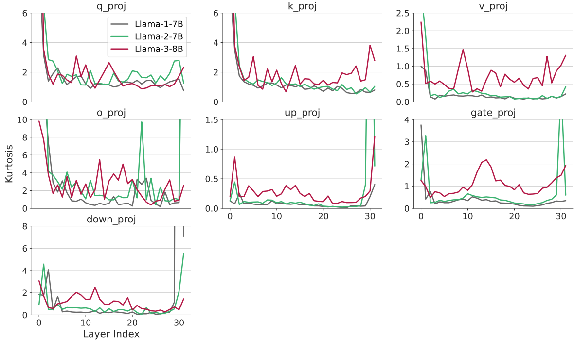
Figure B.1: The kurtosis across various layers in different Llama series reveals three key observations: (1) Layers at either the beginning or the end of LLMs tend to exhibit higher kurtosis values; (2) In the majority of layers, the kurtosis follows a consistent trend across Llama series, with Llama-3 showing the highest values, followed by Llama-2, and then Llama-1; (3) Different types of layers display varying scales of kurtosis, suggesting that a bit allocation strategy that accounts for quantization difficulty could yield better results. We leave the exploration of this idea to future work.
