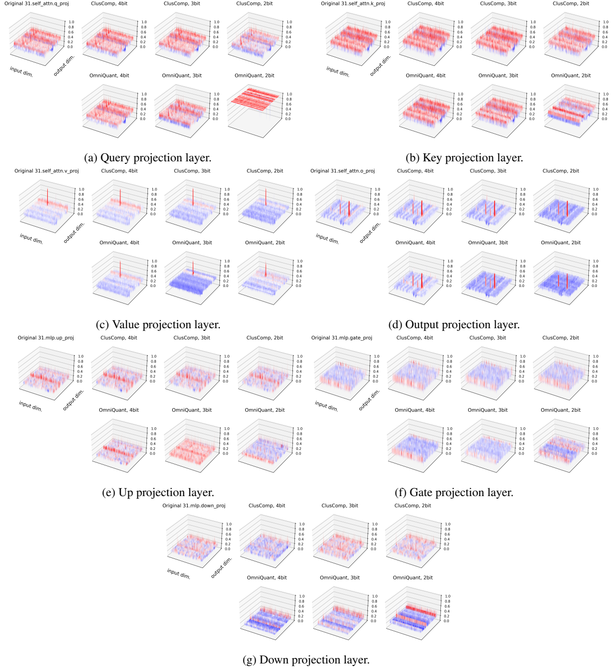
Figure A.4: Weight patterns of all layers in the last block (31-st block) of Llama-2-7B. Darker red and blue indicate larger and smaller weight values, respectively. ClusComp’s weight distribution of different bit levels can better simulate the original weight distribution.
