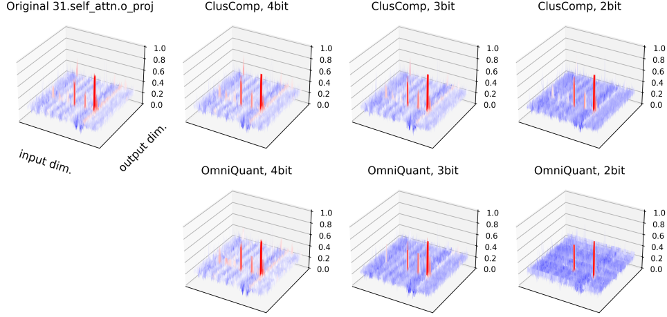
Figure 4: Weight patterns of a cherry-picked layer in Llama-2-7B. Darker red and blue indicate larger and smaller weight values, respectively. Please refer to §A.4 for the visualization setting and the visualization of more layers.
