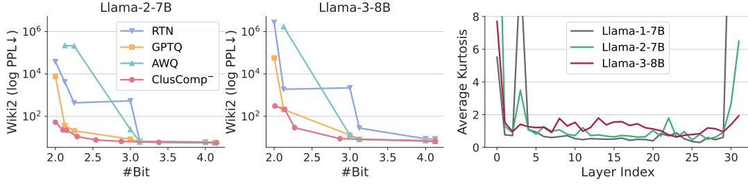
Figure 2: The Llama series becomes progressively harder to quantize. Left & Middle: From Llama-2 to Llama-3, all methods struggle more with lower-bit quantization, though ClusComp + is the least affected. Right: From Llama-1 to Llama-3, the average weight kurtosis across most layers increases.
