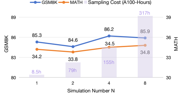
Figure 4: Accuracy of MetaMath-Mistral-7B-Full-Step-DPO using BoN decoding with K = 15 . The PRM uses a fixed sampling number M = 32 , while the simulation number N varies. Purple bars indicate the A100-Hours cost for constructing PRM training data.
