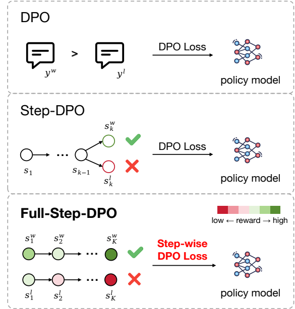
Figure 1: Comparison between DPO, Step-DPO, and our Full-Step-DPO . DPO operates on solution-wise preference data. Step-DPO advances to step-wise data but optimizes only a single step. Full-Step-DPO optimizes all steps with a novel step-wise DPO loss, effectively enhancing the model’s reasoning capability.
