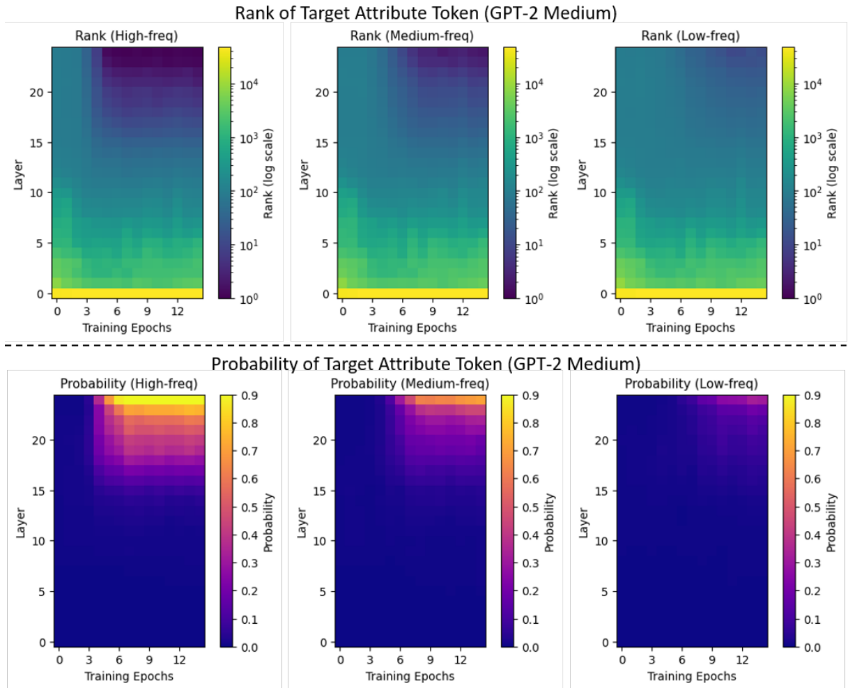
Figure 16: Top: Rank of the target attribute token when unembedding the intermediate layer’s output into vocabulary space at the last token position throughout training for GPT-2 Medium. Bottom: Probability of the target attribute token when unembedding the intermediate layer’s output into vocabulary space at the last token position throughout training for GPT-2 Medium. Low-freq, Medium-freq, and High-freq represent knowledge with frequencies in the ranges [1, 2) , [2, 5] and (5, 27] , respectively.
