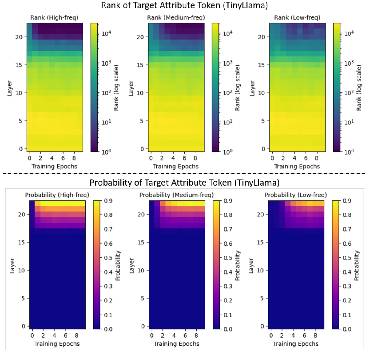
Figure 17: Top: Rank of the target attribute token when unembedding the intermediate layer’s output into vocabulary space at the last token position throughout training for TinyLlama. Bottom: Probability of the target attribute token when unembedding the intermediate layer’s output into vocabulary space at the last token position throughout training for TinyLlama. Low-freq, Medium-freq, and High-freq represent knowledge with frequencies in the ranges [1, 2) , [2, 5] and (5, 27] , respectively.
