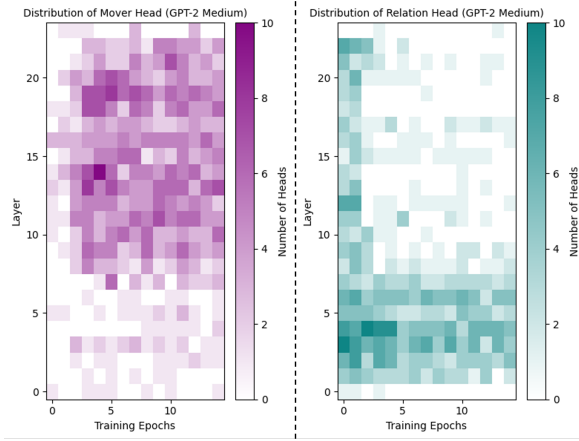
Figure 13: Left: Layer distribution of mover head in the knowledge circuits in GPT-2 Medium throughout training. Right: Layer distribution of relation head in the knowledge circuits in GPT-2 Medium throughout training.
