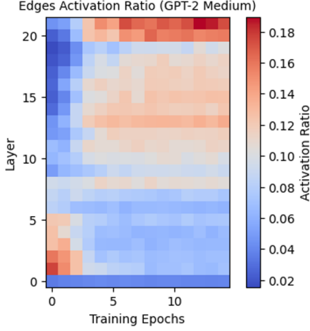
Figure 12: Layer distribution of the edges activation ratio within the knowledge circuits in GPT-2 Medium.
