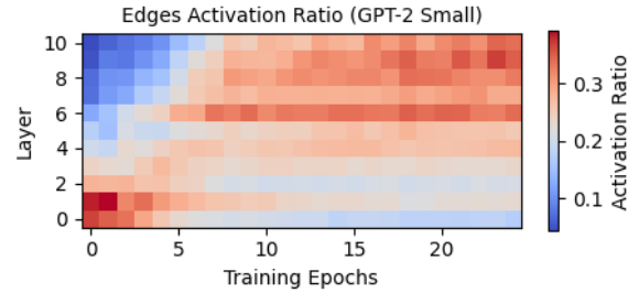
Figure 7: Layer distribution of the edges activation ratio within the knowledge circuits in GPT-2 Small.
