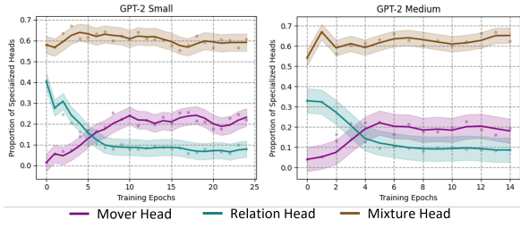
Figure 5: Proportion of specialized attention heads in all nodes of the knowledge circuits throughout training for GPT-2 Small and GPT-2 Medium. Note that we smooth the curves using a window size of 3 epochs.
