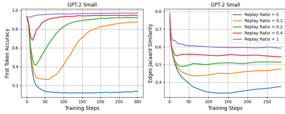
Figure 14: Edges Jaccard Similarity of intermediate knowledge circuits with the circuits at the final checkpoint of the previous knowledge acquisition experiment.
