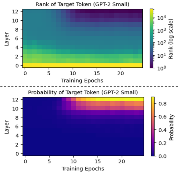
Figure 8: Top: Rank of the target attribute token when unembedding the intermediate layer’s output into vocabulary space at the last token position throughout training for GPT-2 Small. Bottom: The corresponding probability of the target attribute token .
