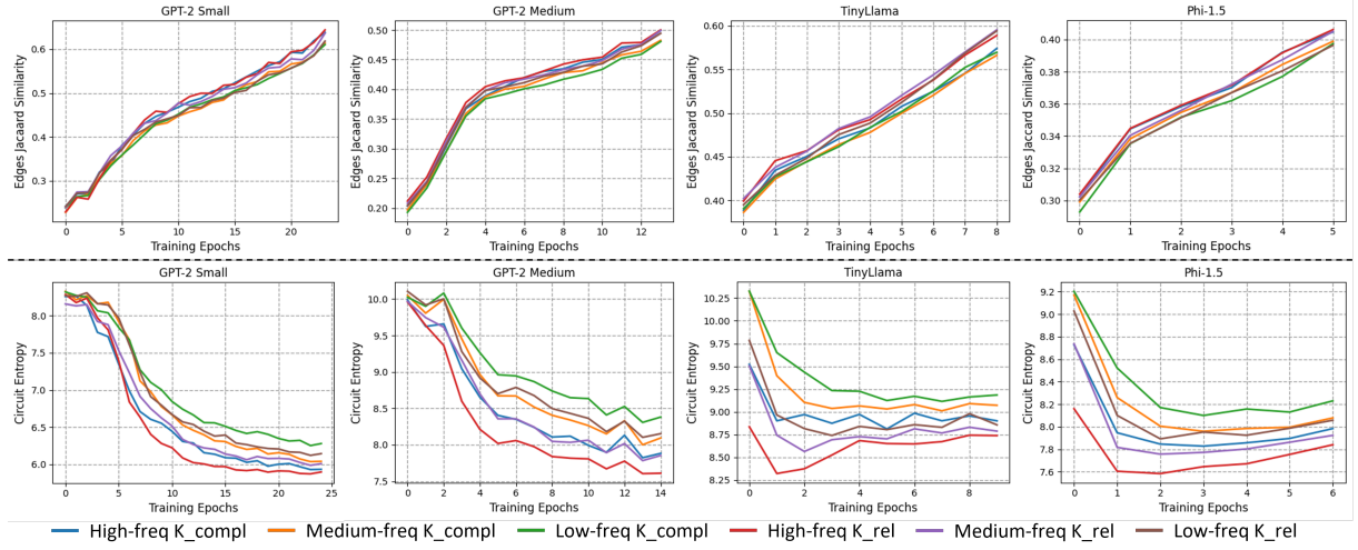
Figure 3: Top: Edges Jaccard Similarity of intermediate knowledge circuits with the circuits at the final checkpoint. Bottom: Knowledge Cutcuit Entropy of knowledge circuits throughout training. K_rel and K_compl represent relevant new knowledge and completely new knowledge, respectively. Low-freq, Medium-freq, and High-freq represent knowledge with frequencies in the ranges [1, 2) , [2, 5] and (5, 27] , respectively.
