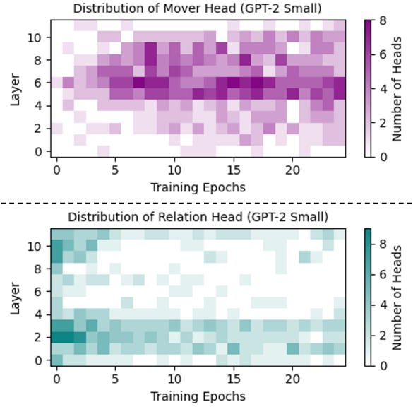
Figure 6: Top: Layer distribution of mover head in the knowledge circuits in GPT-2 Small throughout training. Bottom: Layer distribution of relation head in the knowledge circuits in GPT-2 Small throughout training.
