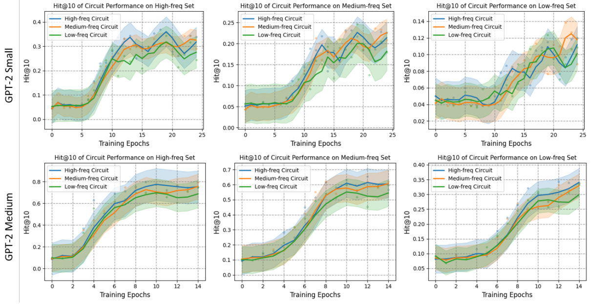
Figure 10: Hit@10 of the transfer performance of knowledge circuits in GPT-2 Small and GPT-2 Medium throughout training. Low-freq Circuit, Medium-freq Circuit, and High-freq Circuit represent knowledge circuits identified by knowledge with the frequencies in the ranges [1, 2) , [2, 5] and (5, 27] , respectively. Note that we smooth the curves using a window size of 3 epochs for all settings.
