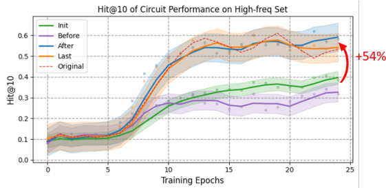
Figure 4: Hit@10 of the performance of aligned knowledge circuits in GPT-2 Small throughout training. Init, Before, After, Last represents the circuits whose topologies align with those at the initial checkpoint, the checkpoint before the phase shift, the checkpoint after the phase shift, and the last checkpoint, respectively. Original represents the original knowledge circuits at each checkpoint. Note that we smooth the curves using a window size of 3 epochs.
