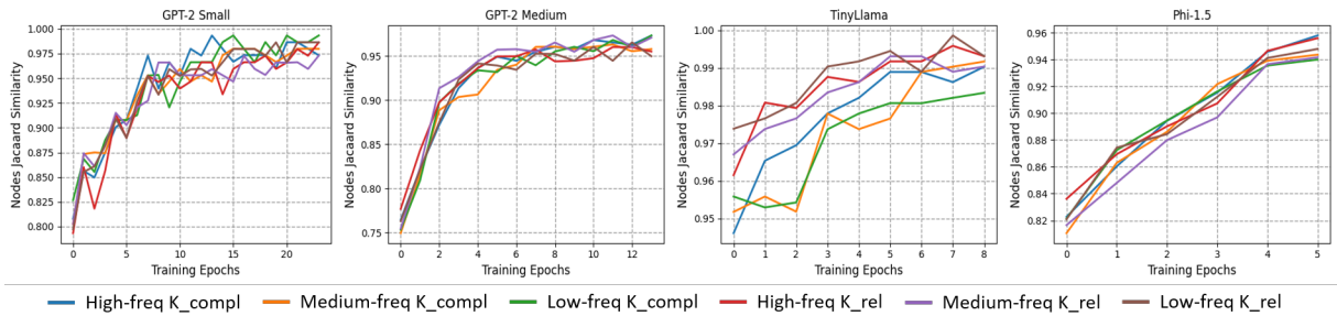
Figure 11: Nodes Jaccard Similarity of intermediate knowledge circuits with the circuits at the final checkpoint. K_rel and K_compl represent relevant new knowledge and completely new knowledge, respectively. Low-freq, Medium-freq, and High-freq represent knowledge with frequencies in the ranges [1, 2) , [2, 5] and (5, 27] , respectively.
