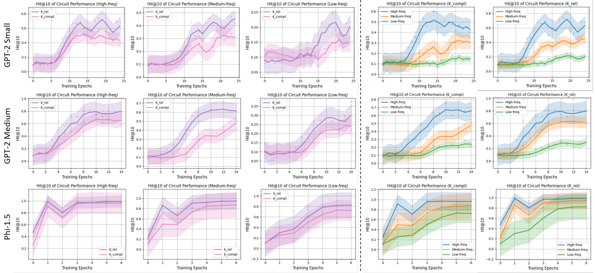
Figure 2: Hit@10 of the performance of knowledge circuits in GPT-2 Small, GPT-2 Medium and Phi-1.5 throughout training. Left: Performance for circuits discovered by different types of knowledge, where K_{rel} and K_{comp1} represent relevant new knowledge and completely new knowledge , respectively. Right: Performance for circuits discovered by different frequencies of knowledge, where Low-freq , Medium-freq , and High-freq represent knowledge with frequencies in the ranges [1, 2) , [2, 5] and (5, 27] , respectively. Note that we smooth the curves using a window size of 3 epochs for all settings.
