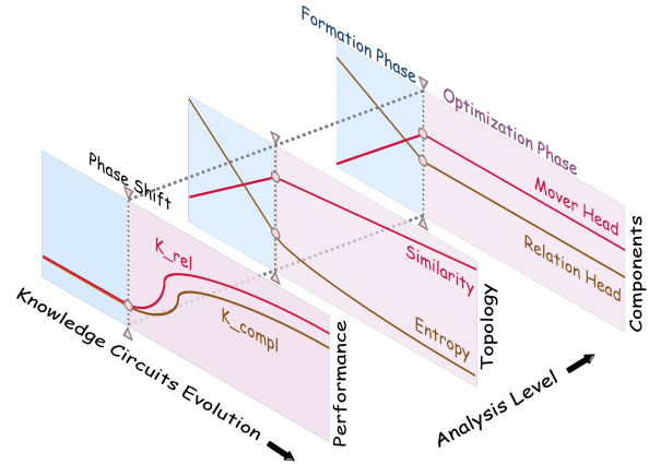
Figure 1: Illustration of our findings: Phase shift from formation to optimization in the evolution of knowledge circuits, each phase characterized by distinct features at the performance, topology, and component levels.
