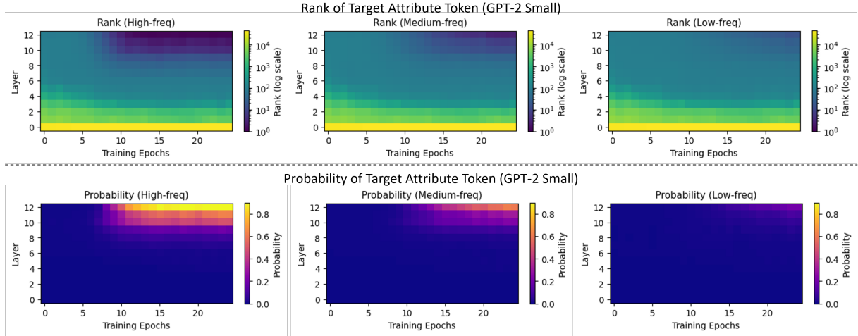
Figure 15: Top: Rank of the target attribute token when unembedding the intermediate layer’s output into vocabulary space at the last token position throughout training for GPT-2 Small. Bottom: Probability of the target attribute token when unembedding the intermediate layer’s output into vocabulary space at the last token position throughout training for GPT-2 Small. Low-freq, Medium-freq, and High-freq represent knowledge with frequencies in the ranges [1, 2) , [2, 5] and (5, 27] , respectively.
