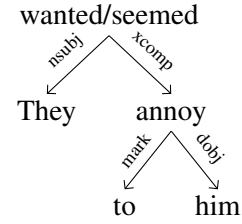
Figure 3: Dependency parse for the two sentences "They seemed/wanted to annoy him." The two trees are identical, and the distance between the subject and embedded verb is 2 while the distance between the subject and the infinitive or direct object is 3. This is true even if one were to use extended Universal Dependencies, which also conflates SC and SR verbs.
