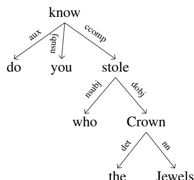
Figure 2: Above are two different sentences that yield identical dependency parses. While similar, the sentences have different meanings (imagine you are being questioned about the theft of the Crown Jewels: the first question merely seeks to inquire whether or not you know who the thief is, while the latter presumes you know who the thief is and seeks to learn the identity). This illustrates both the ways in which dependency trees do not capture linear order, and highlights some of the limitations of dependency trees.
