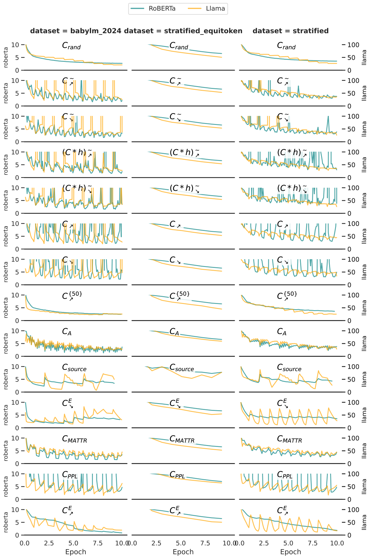
Figure 12: Training loss trajectories under different curricula.
