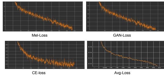
Figure 2: Loss plots
