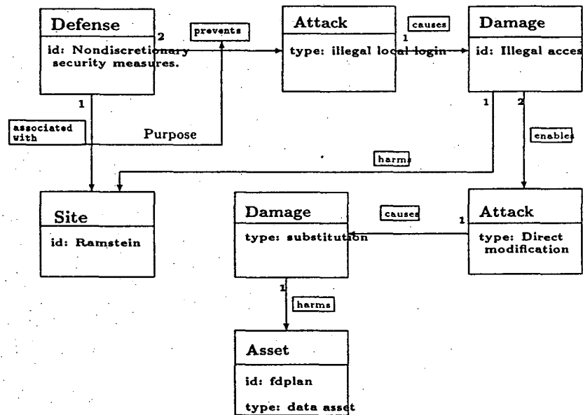
Figure 2: The content representation graph (instantiated domain model) for the example, representing the full CDK
