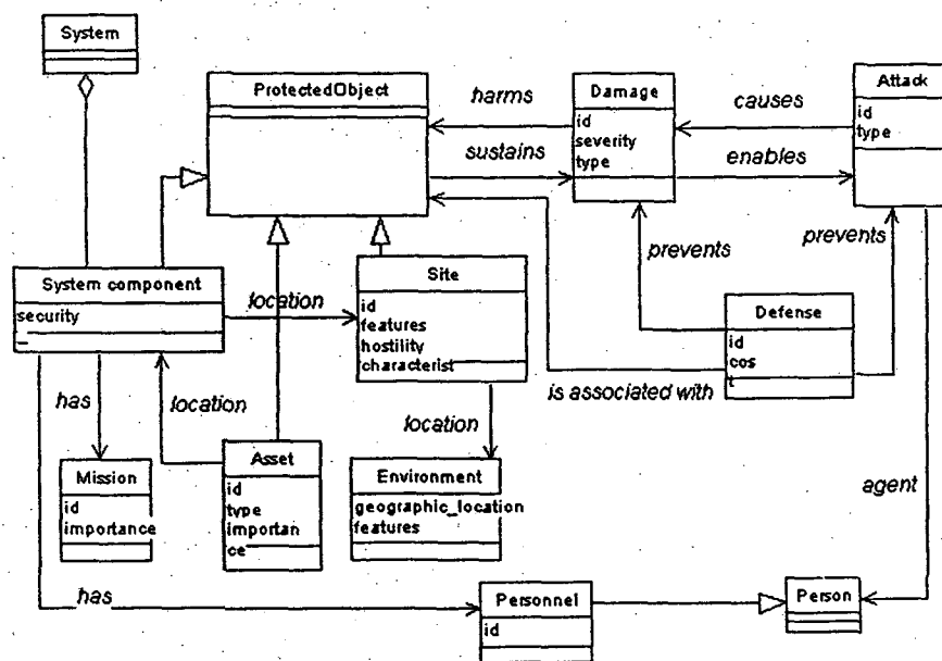
Figure 1: The domain model
