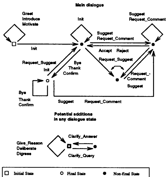
Figure 1: A dialogue model for the description of appointment scheduling dialogs
