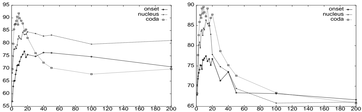
Figure 4: Evaluation on pseudo-disambiguation task for English (left) and German (right)
