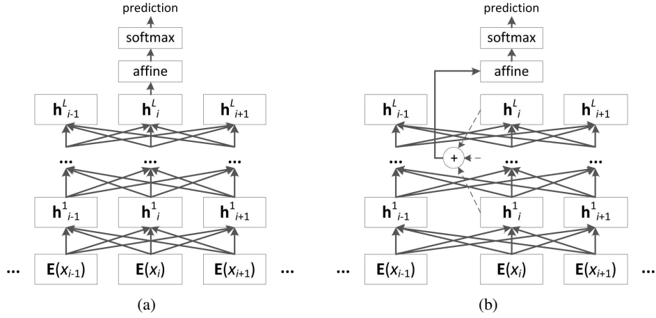
Figure 1: Illustration of WSD models by linear projection of (a) the last layer and (b) the weighted sum of all layers.
