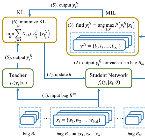
Figure 2: The training process of NITE-NER.
