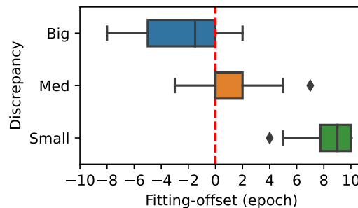
Figure 6: Fitting-offset of tokens grouped by prediction discrepancy .
