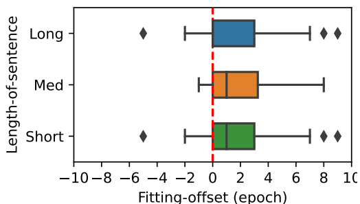
Figure 9: Fitting-offset of tokens grouped by length-of-sentence .
