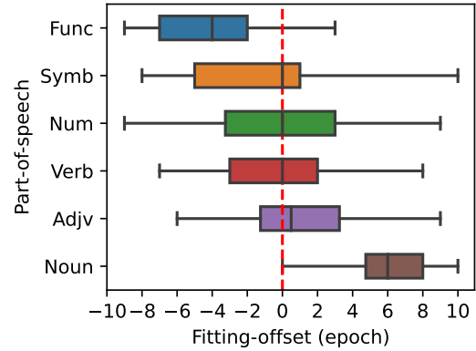
Figure 4: Fitting-offset of tokens grouped by parts-of-speech .
