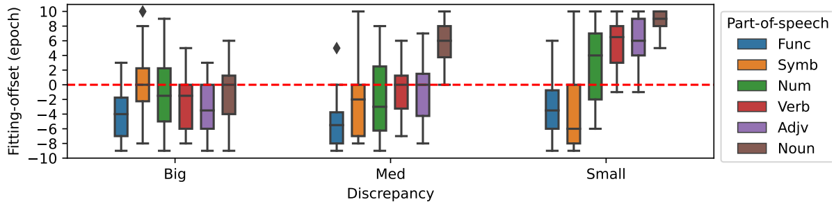
Figure 8: Fitting-offset of tokens grouped by discrepancy and parts-of-speech .
