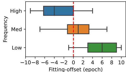
Figure 3: Fitting-offset of tokens grouped by token frequency.
