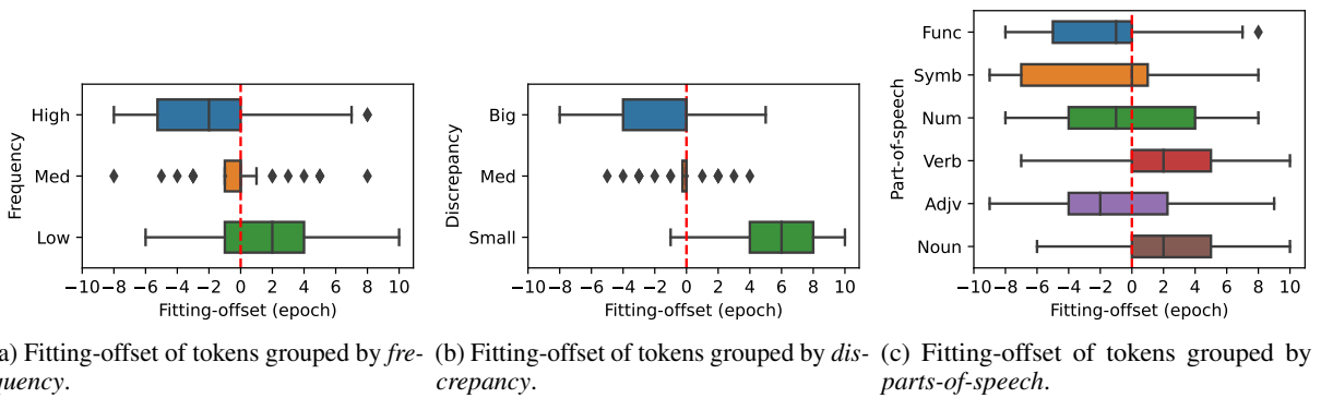
Figure 16: The Domain: Fitting-offset of tokens evaluated on Europarl English-German (250,000 samples).
