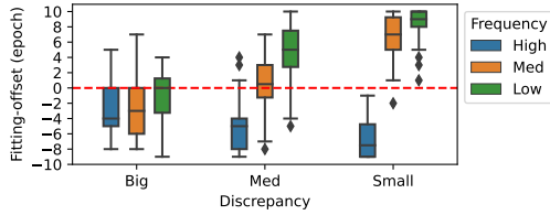
Figure 7: Fitting-offset of tokens grouped by discrepancy and frequency.
