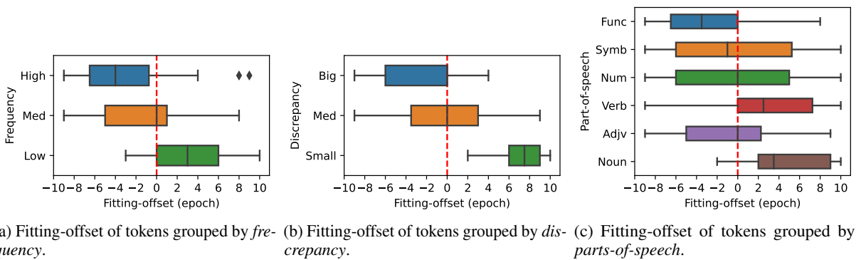
Figure 17: The Data Scale: Fitting-offset of tokens evaluated on Europarl English-German (500,000 samples)..
