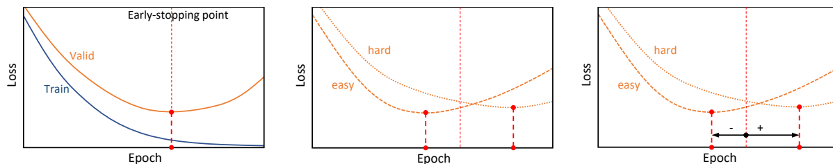
(a) Idealized training and validation loss curves, where the model is selected by early stopping.
