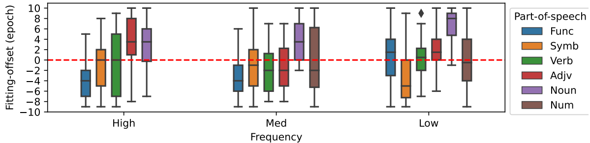
Figure 5: Fitting-offset of tokens grouped by frequency and parts-of-speech .
