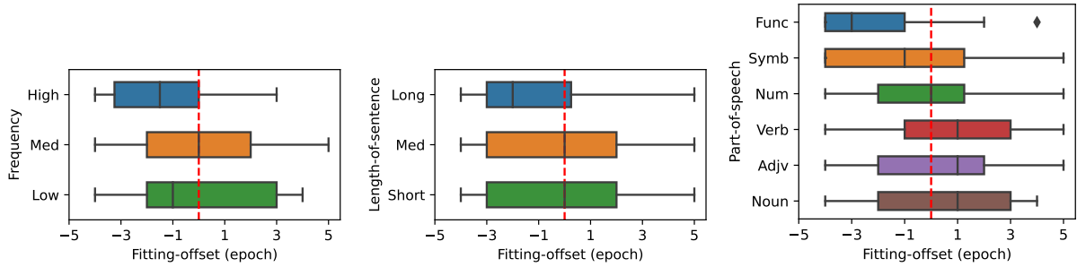
(a) Fitting-offset of tokens grouped by frequency. (b) Fitting-offset of tokens grouped by length-of-sentence. (c) Fitting-offset of tokens grouped by parts-of-speech.
