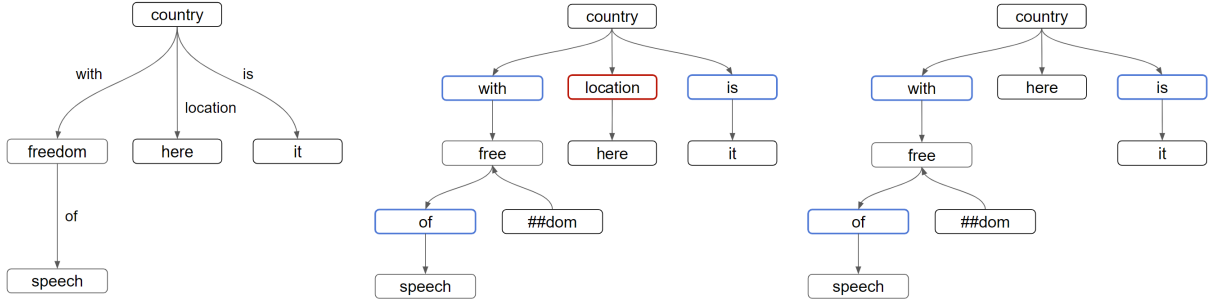
Figure 2: WAG construction of the sentence: "Here, it is a country with the freedom of speech". A graph where AMR concepts are replaced with words (left), a Full WAG (center) and a Contracted WAG (right). Blue lines indicate former AMR relations, and red lines indicate non-aligned nodes. Best seen in color.
