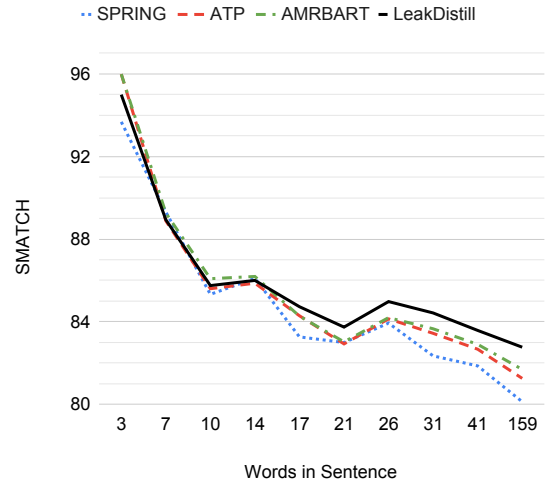
Figure 5: SMATCH score for buckets of 200 instances. X axis shows max. number of words per sentence.
