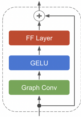
Figure 3: Structural adapter without layer normalization and with GELU activation.
