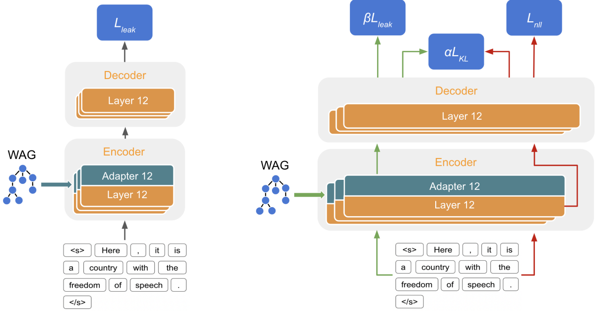
Figure 4: Left: Scheme of the Graph Leakage Model. Right: Scheme of the LeakDistill method with two forward paths: the green path incorporates WAG information via adapters; the red path omits adapters, and it is basically the outcome model for the problem. Consequently, the green path is engaged exclusively during the training phase to guide the red path, while during the inference process, only the red path is operative.
