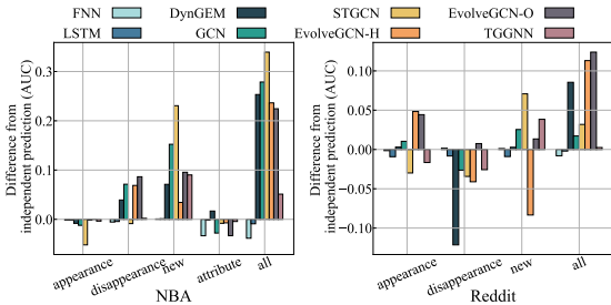
Figure 5: Reuse gain on node loss prediction.
