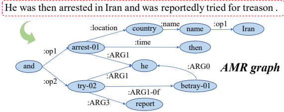
Figure 3: The AMR graph provides abstract and logical semantic information, where the nodes denote the concepts and the edges refer to different relation types. The corresponding text spans for nodes are omitted.
