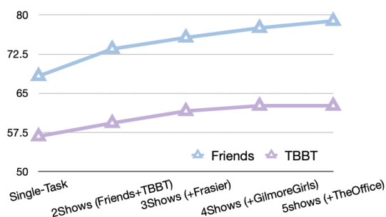
Figure 4: Learning curves of Friends and The Big Bang Theories with increasing training data from other shows.
