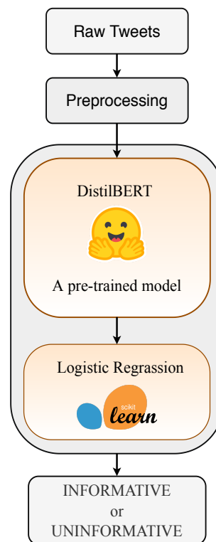
Figure 1: System 2 architecture
