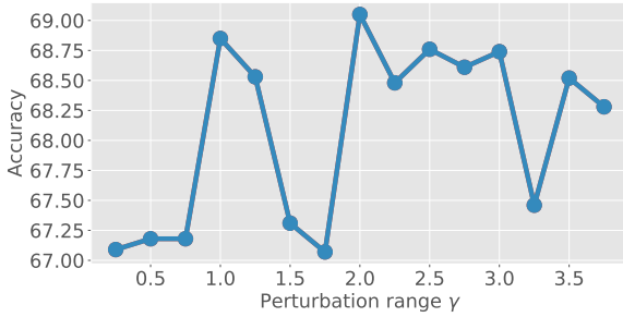
(b) The effect of perturbation range \gamma ( \beta = 8 ).
